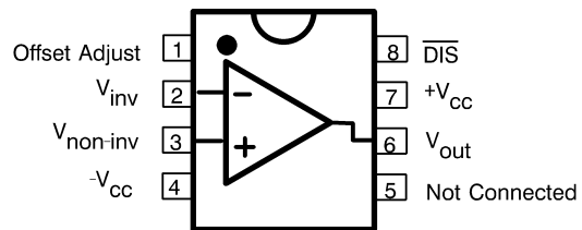
Pinout DIP & SOIC
